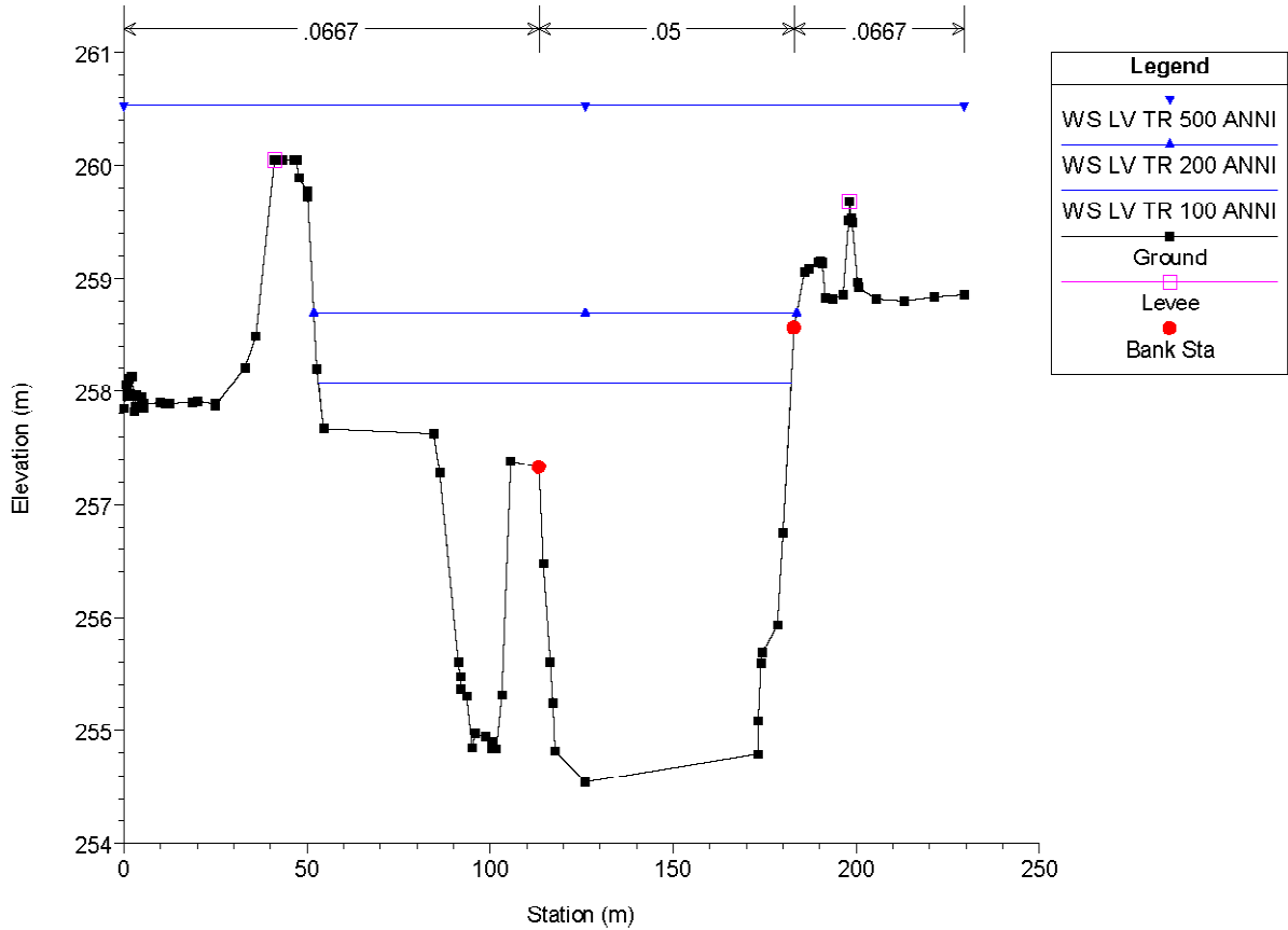
maira 06-02-08 nuove sez Plan: c20_c15 RS = 110 sez int
